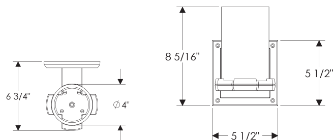
WS410 with E155 Square Designer Escutcheon
