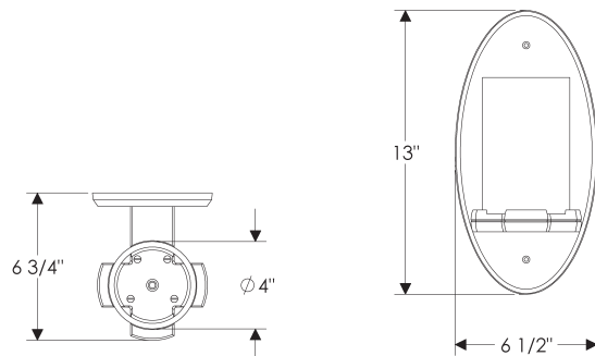
WS410 with E560 Oval Escutcheon
