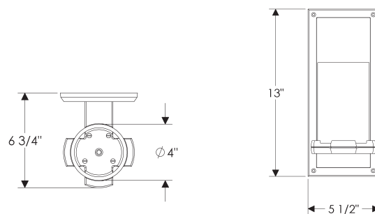
WS410 with G153 Rectangular Designer Escutcheon
