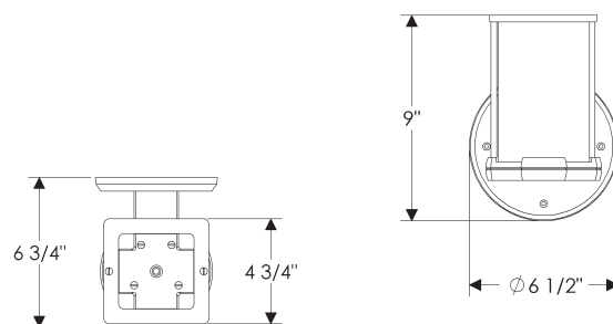
WS418 with E419 Round Escutcheon
