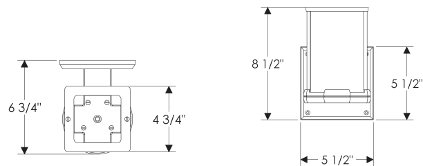
WS418 with E403 Square Escutcheon
