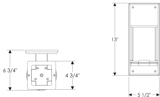
WS418 with G4513 Rectangular Escutcheon
