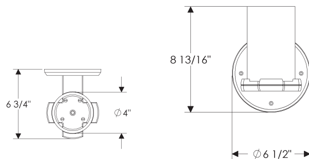
WS410 with E419 Round Escutcheon
