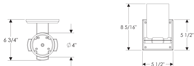
WS410 with E403 Square Escutcheon
