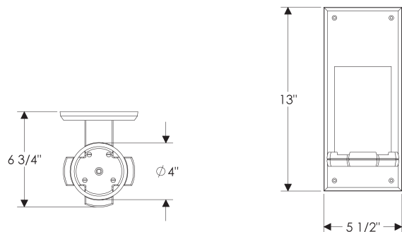
WS410 with G4513 Rectangular Escutcheon
